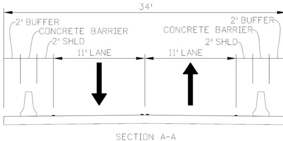
Figure 2: Shoofly Typical Section
